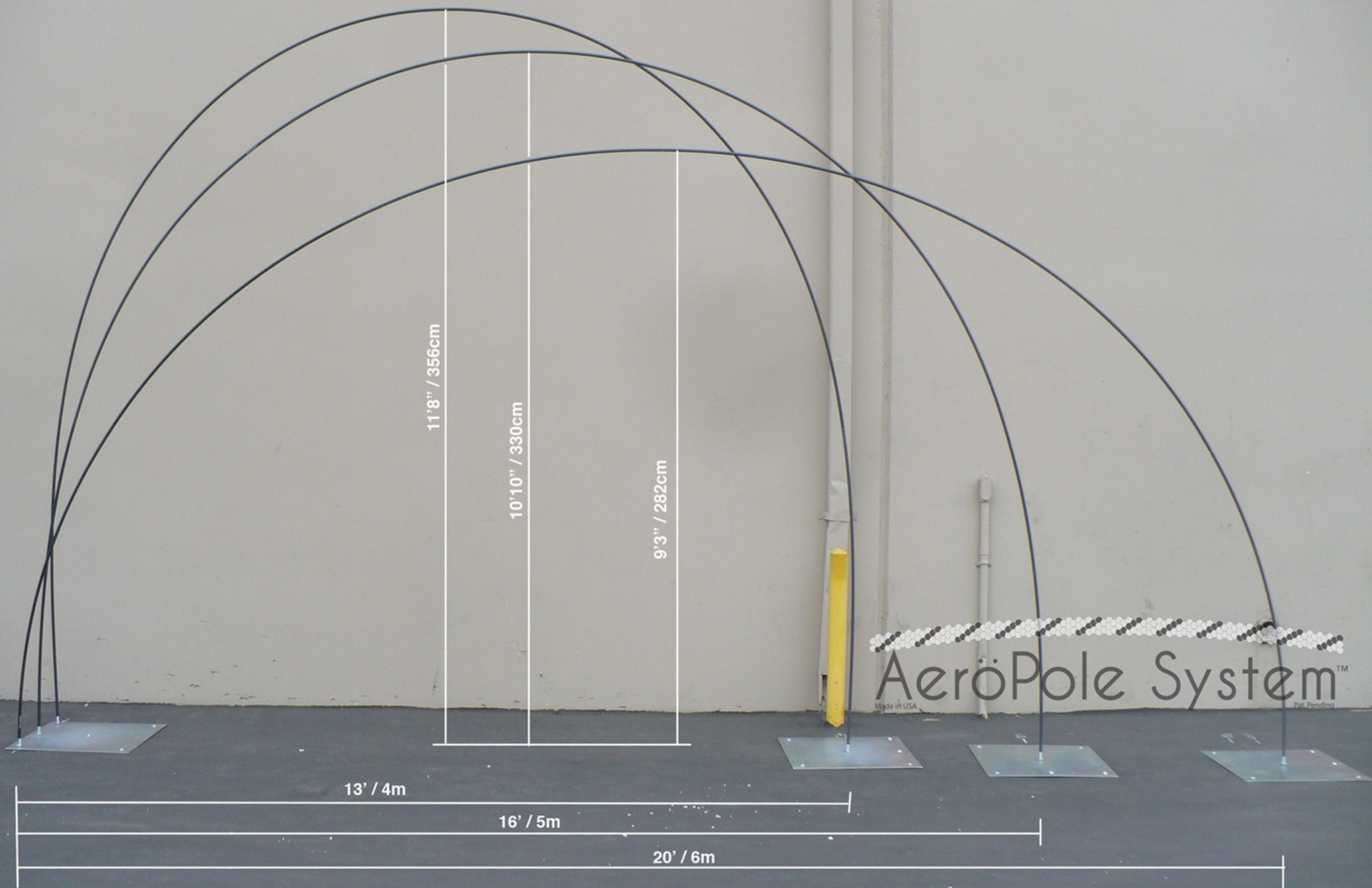
AeroPole System arch with 6 poles.
