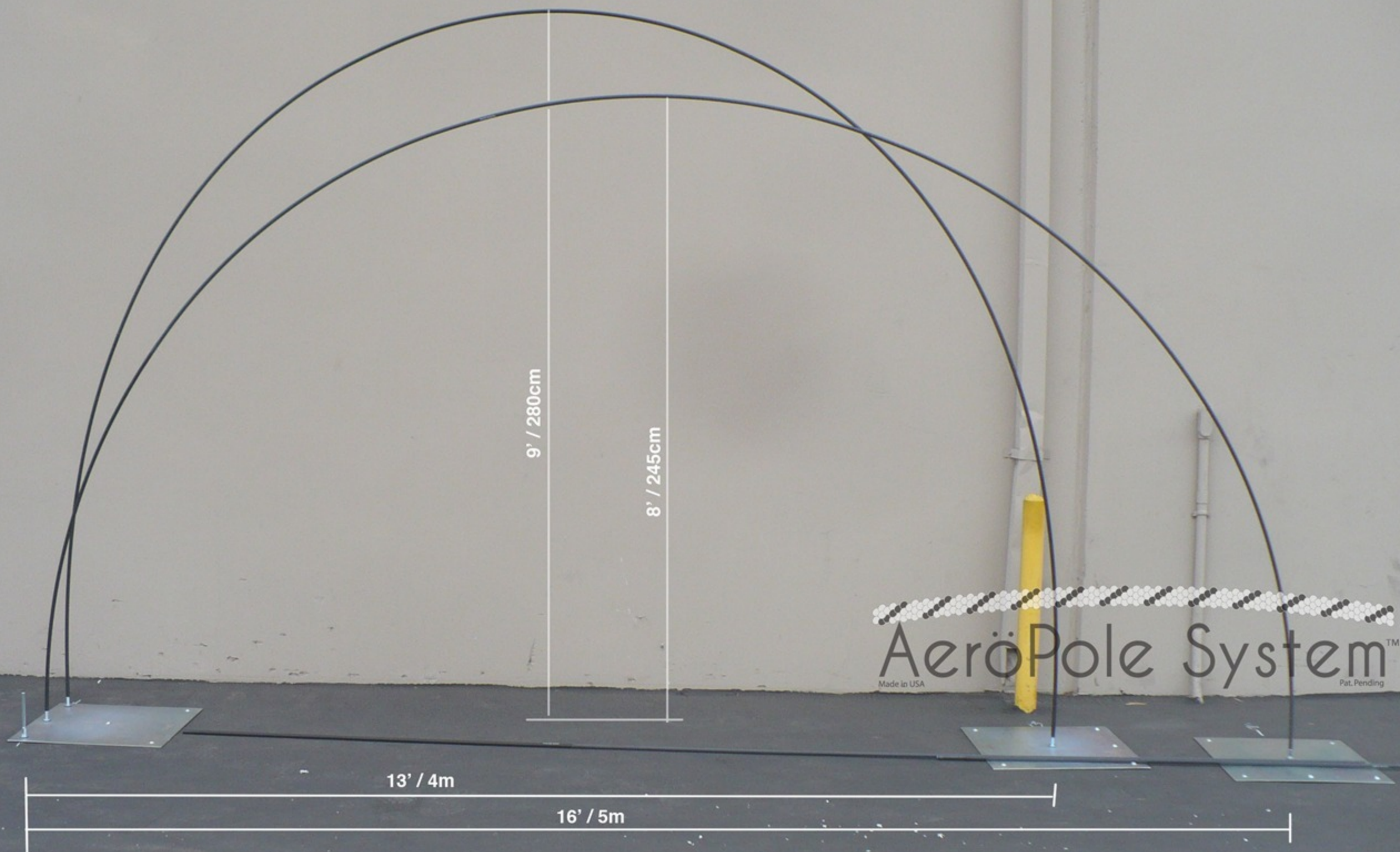
AeroPole System arch with 5 poles.
